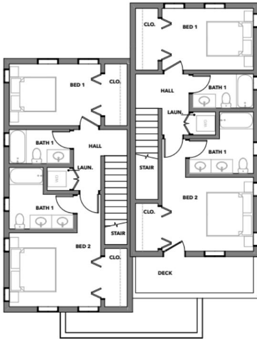
2 UPPER PLAN D 3/16" = 1'-0"
